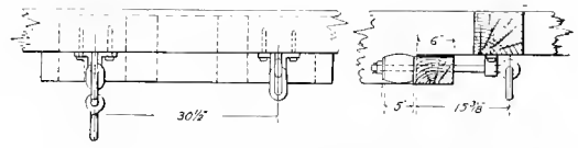
Figs. 1242-1243 Application of Safety chains.
